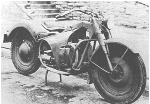
Figure 6. The unorthodox Crosley prototype motorcycle for military testing.
