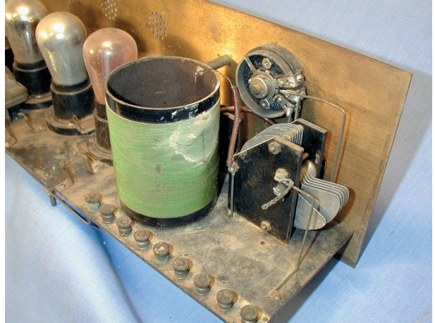
Figure 5. The inside was dirty and the remnants of a dirt dauber's nest can be seen on the side of the tuning coil.
