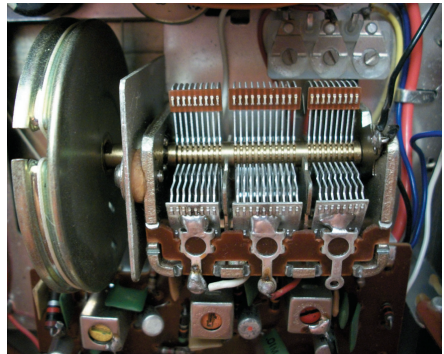
One sign that an RF amplifier is included in an AM radio is to observe that the tuning capacitor has three sections, as in the above picture.
